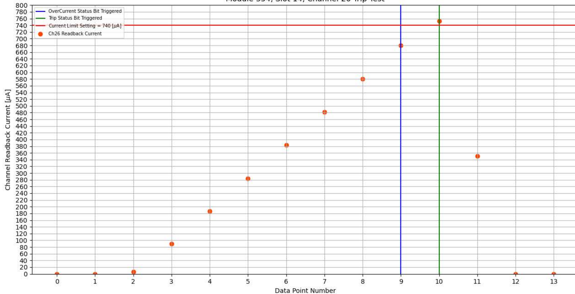
Module 354, Slot 14, Channel 26 Trip Test
