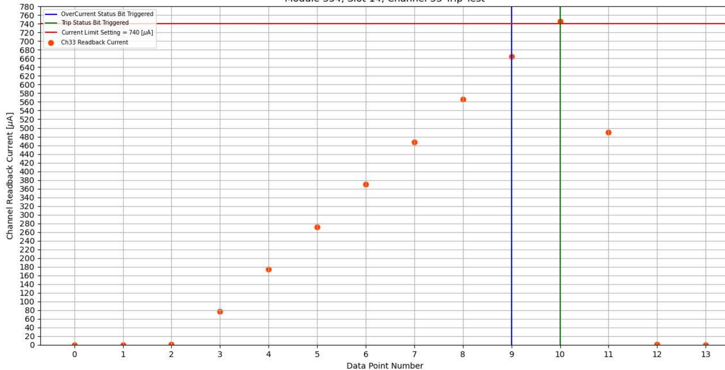
Module 354, Slot 14, Channel 33 Trip Test
