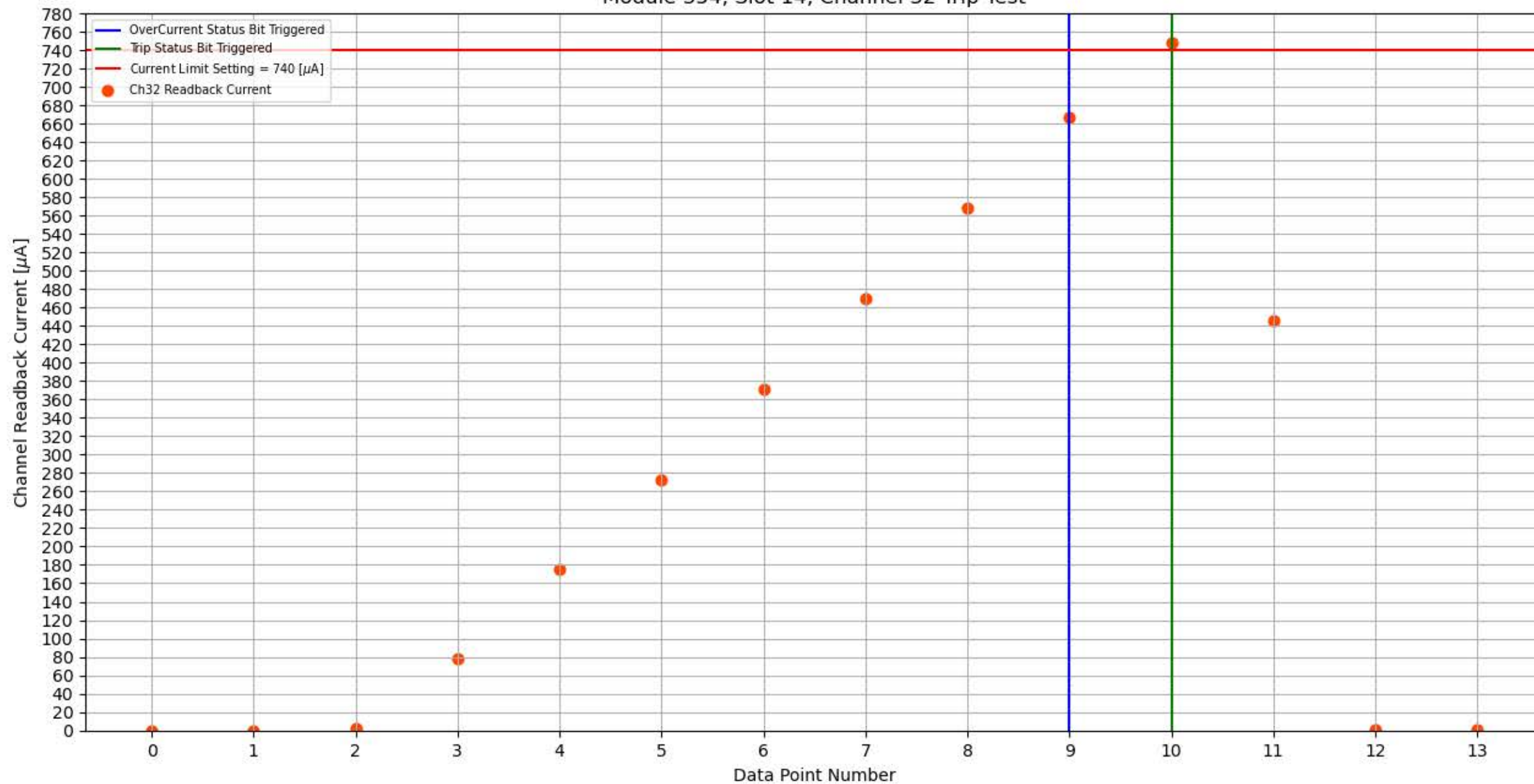
Module 354, Slot 14, Channel 32 Trip Test
