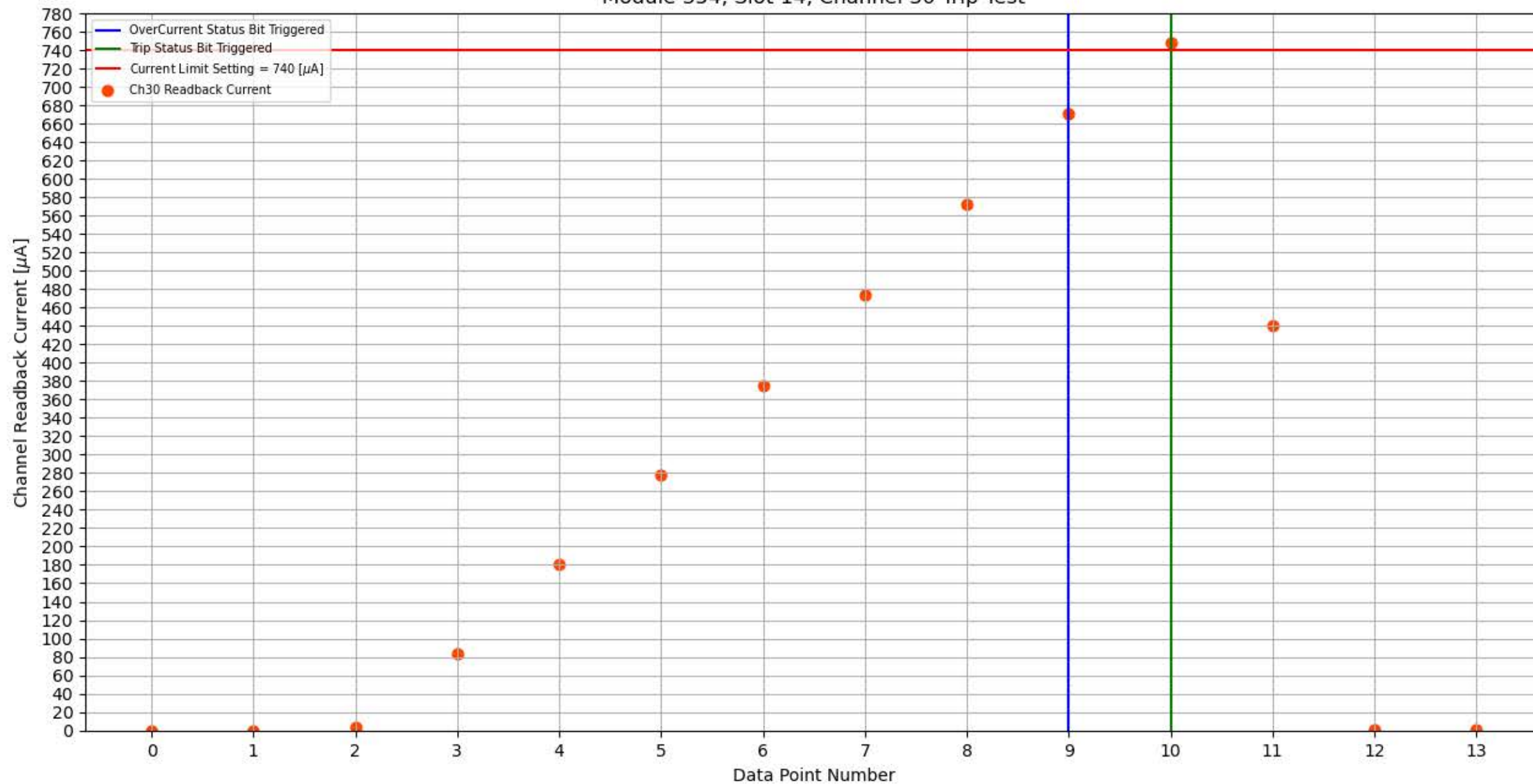
Module 354, Slot 14, Channel 30 Trip Test
