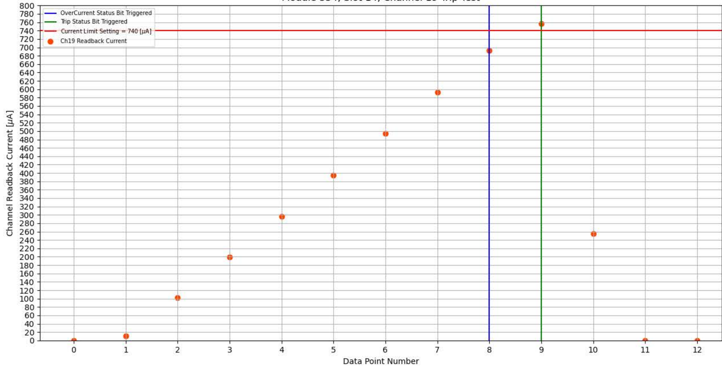
Module 354, Slot 14, Channel 19 Trip Test
