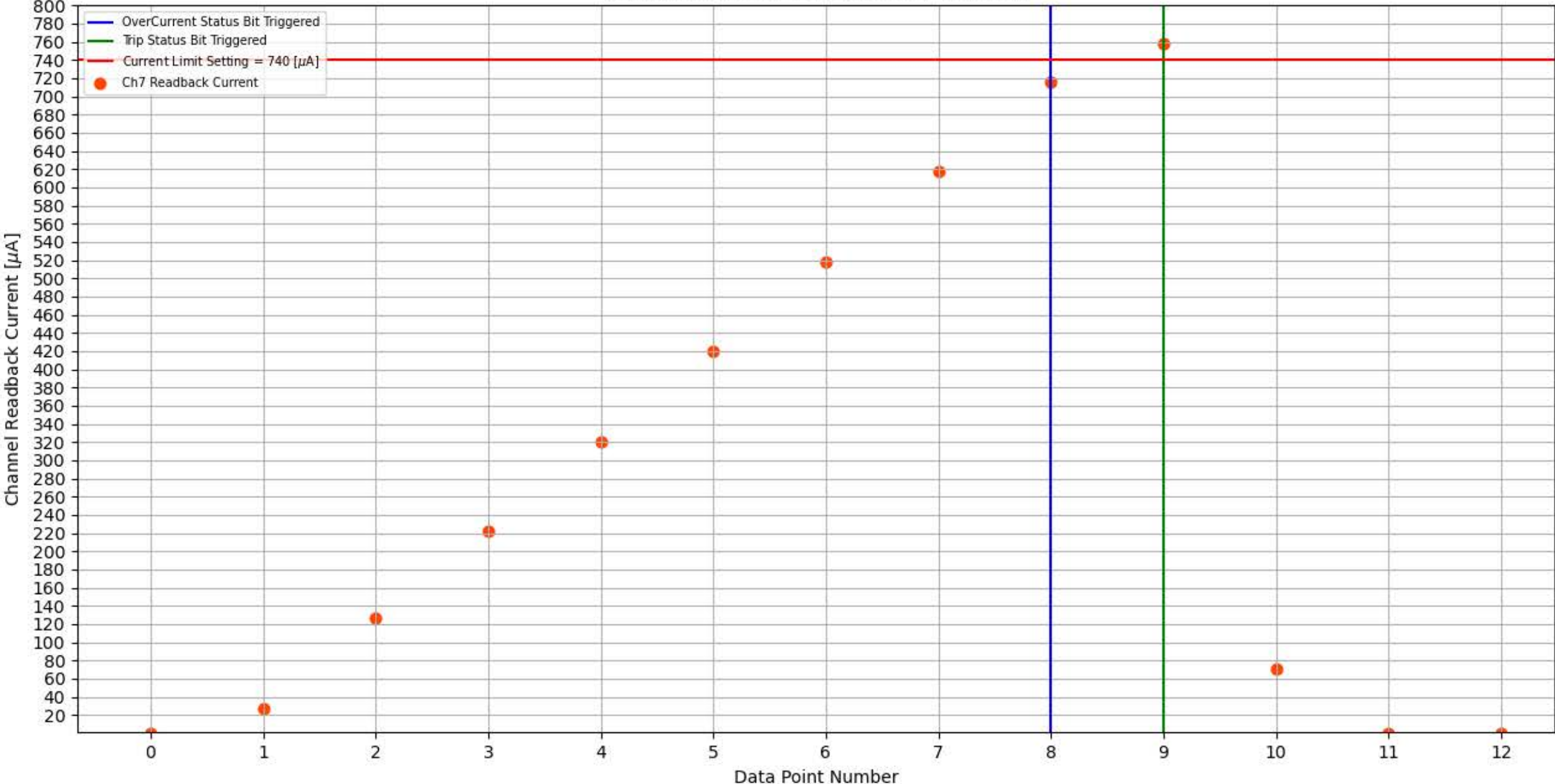
Module 354, Slot 14, Channel 7 Trip Test
