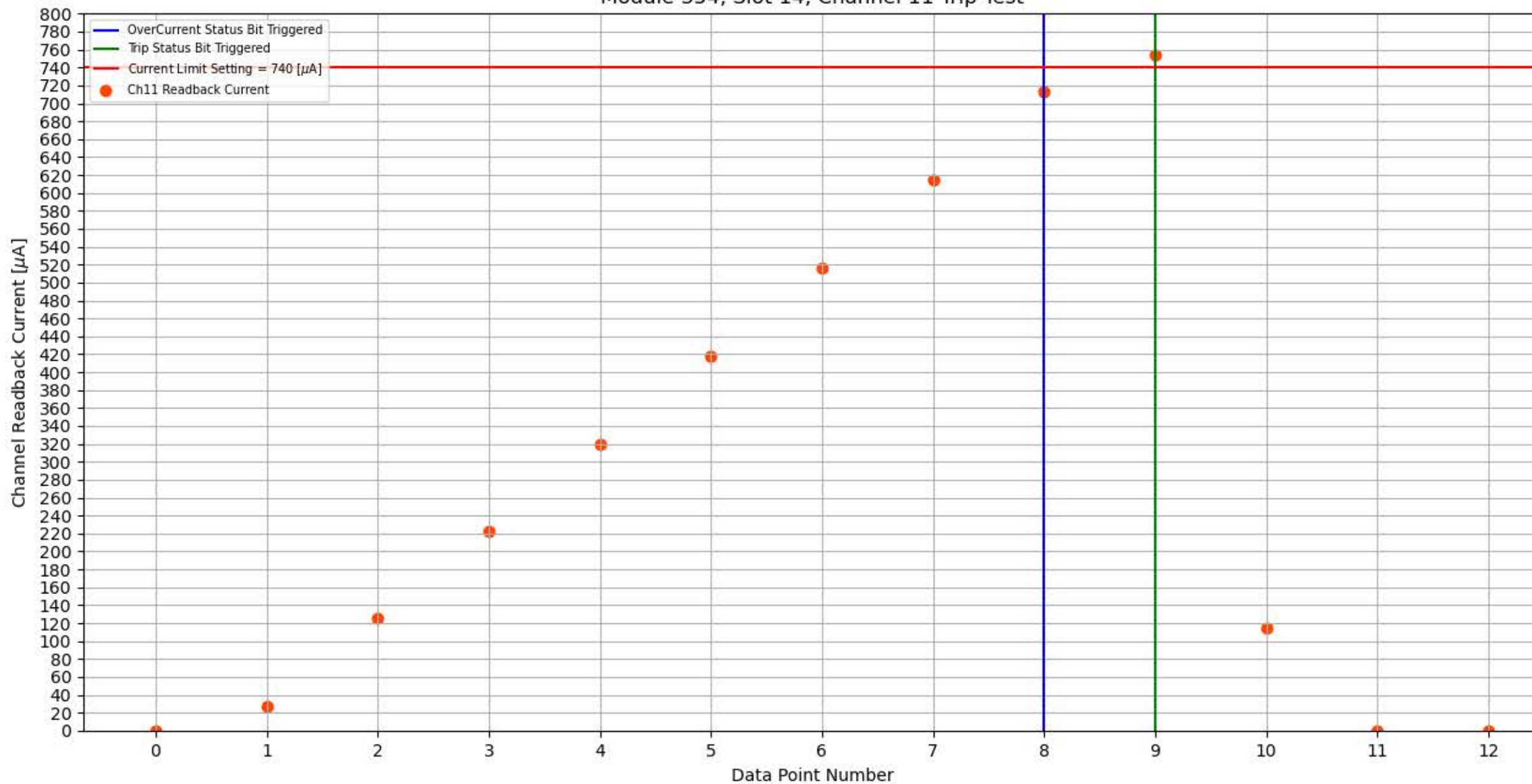
Module 354, Slot 14, Channel 11 Trip Test
