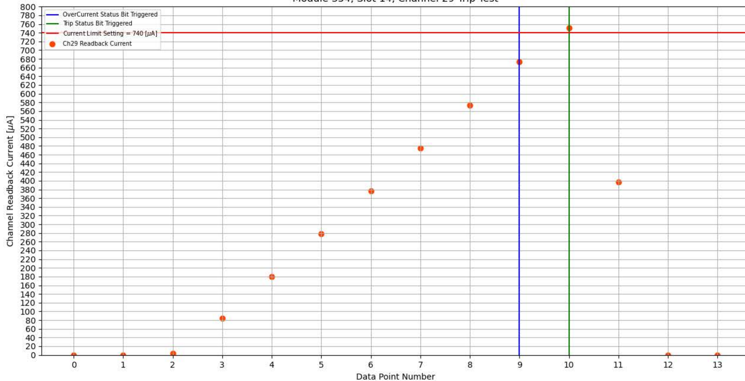
Module 354, Slot 14, Channel 29 Trip Test
