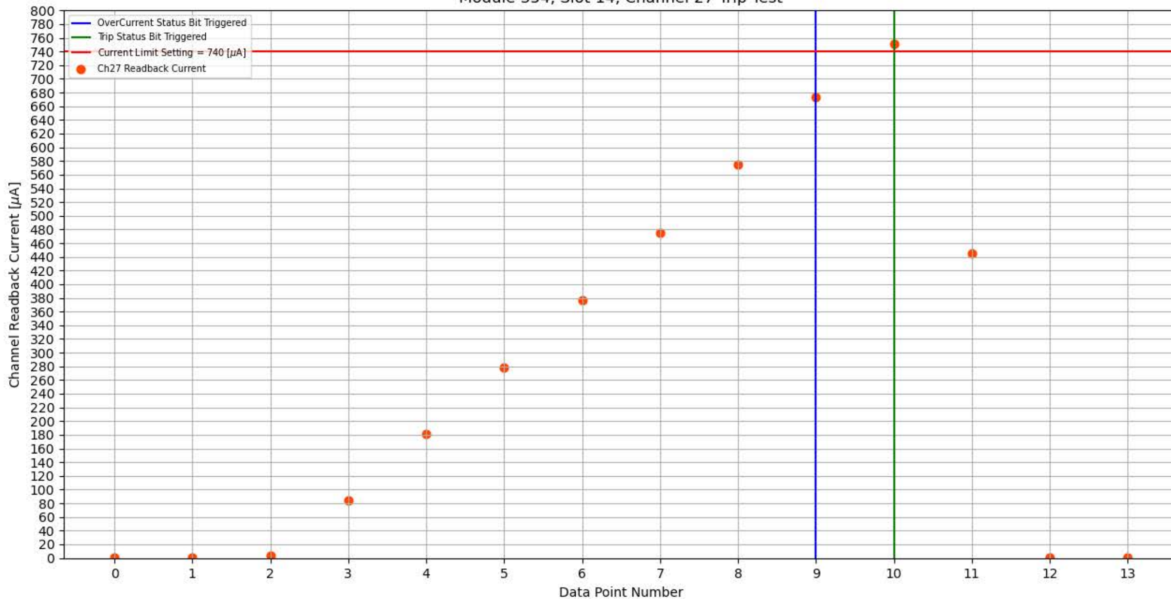
Module 354, Slot 14, Channel 27 Trip Test
