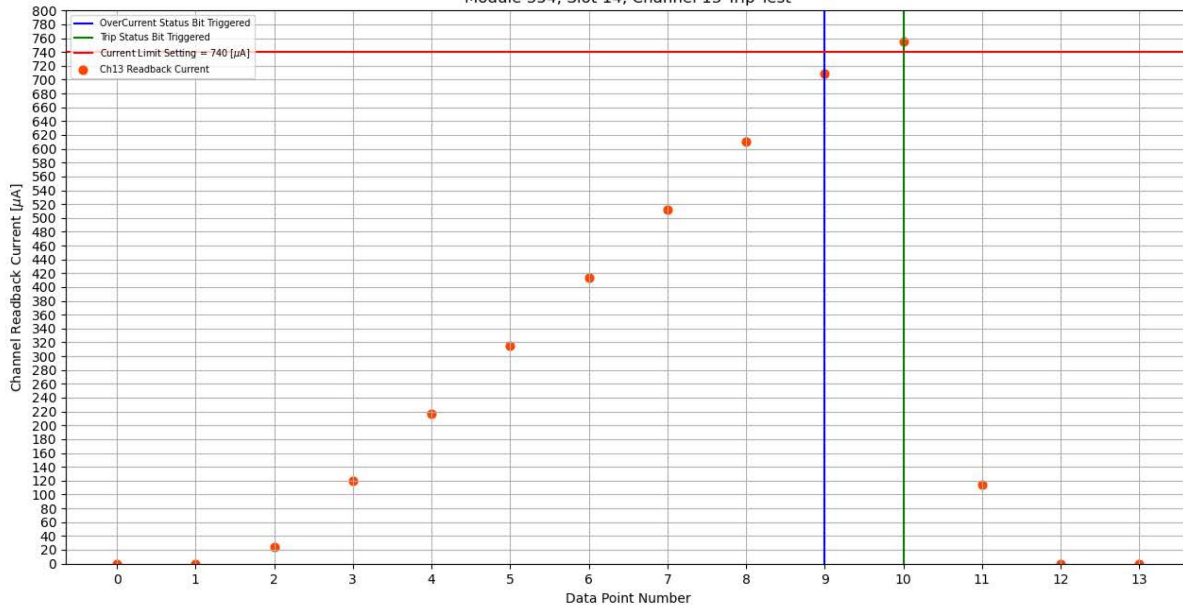
Module 354, Slot 14, Channel 13 Trip Test
