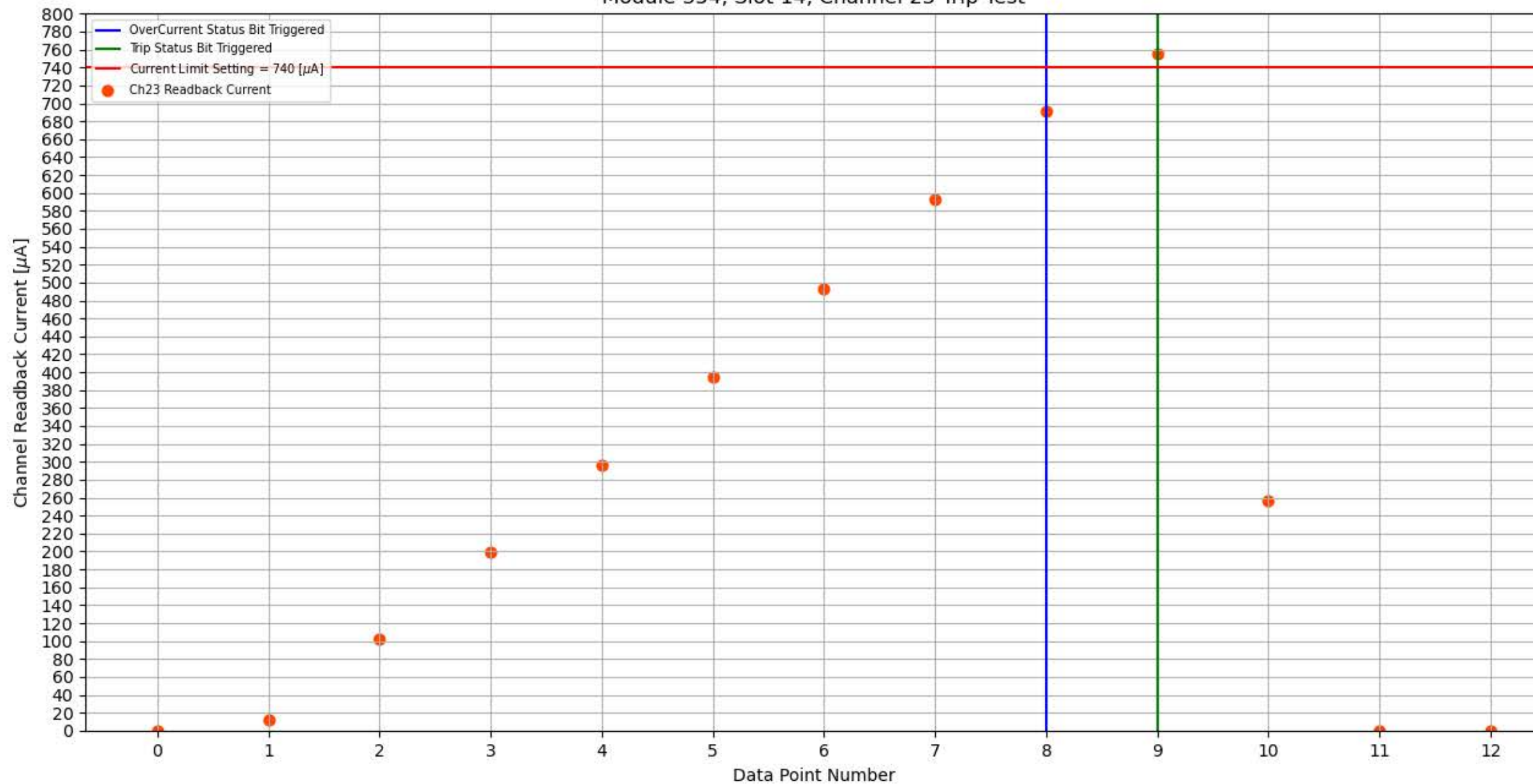
Module 354, Slot 14, Channel 23 Trip Test
