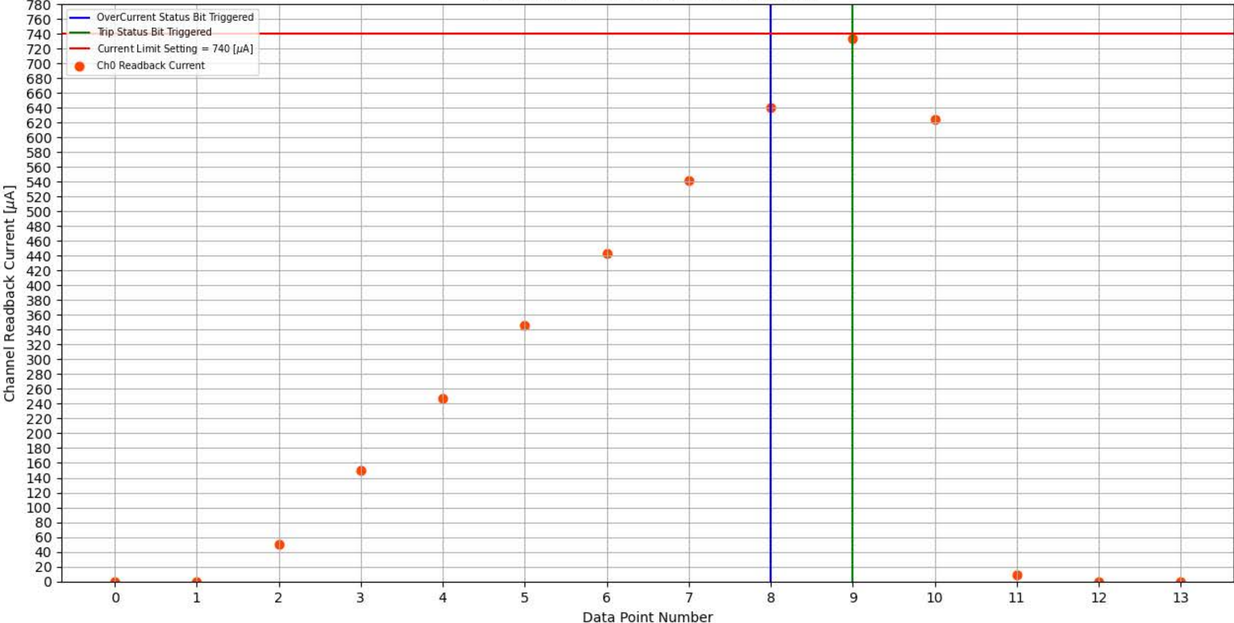
Module 354, Slot 14, Channel 0 Trip Test
