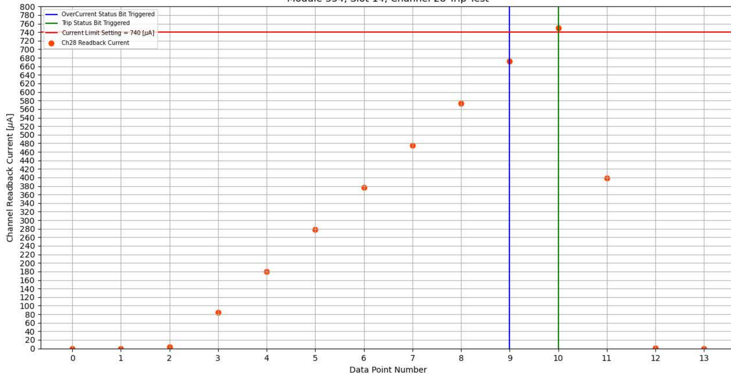
Module 354, Slot 14, Channel 28 Trip Test
