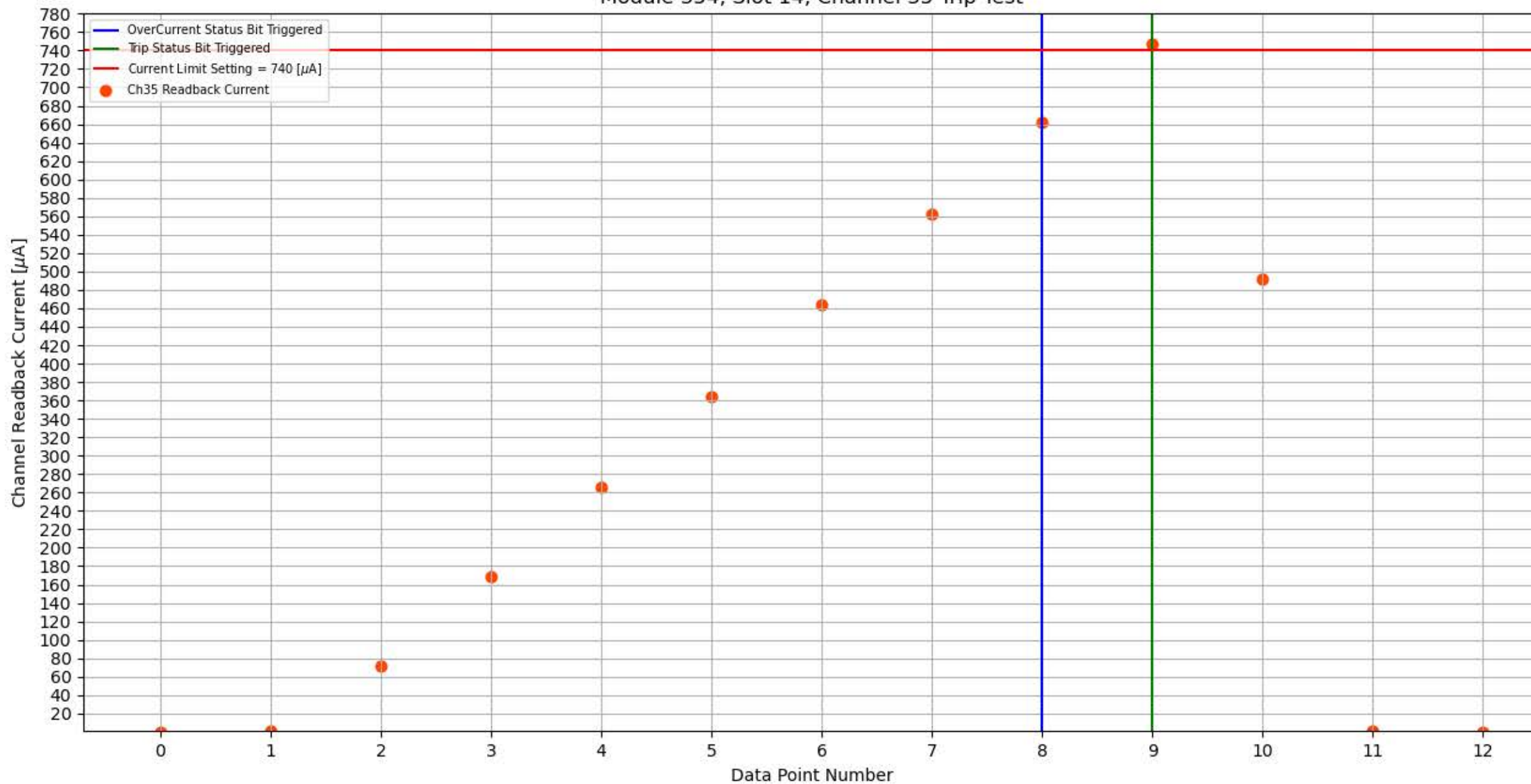
Module 354, Slot 14, Channel 35 Trip Test
