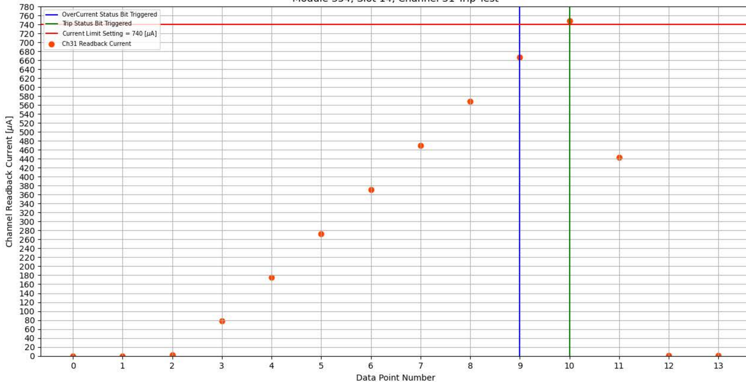
Module 354, Slot 14, Channel 31 Trip Test
