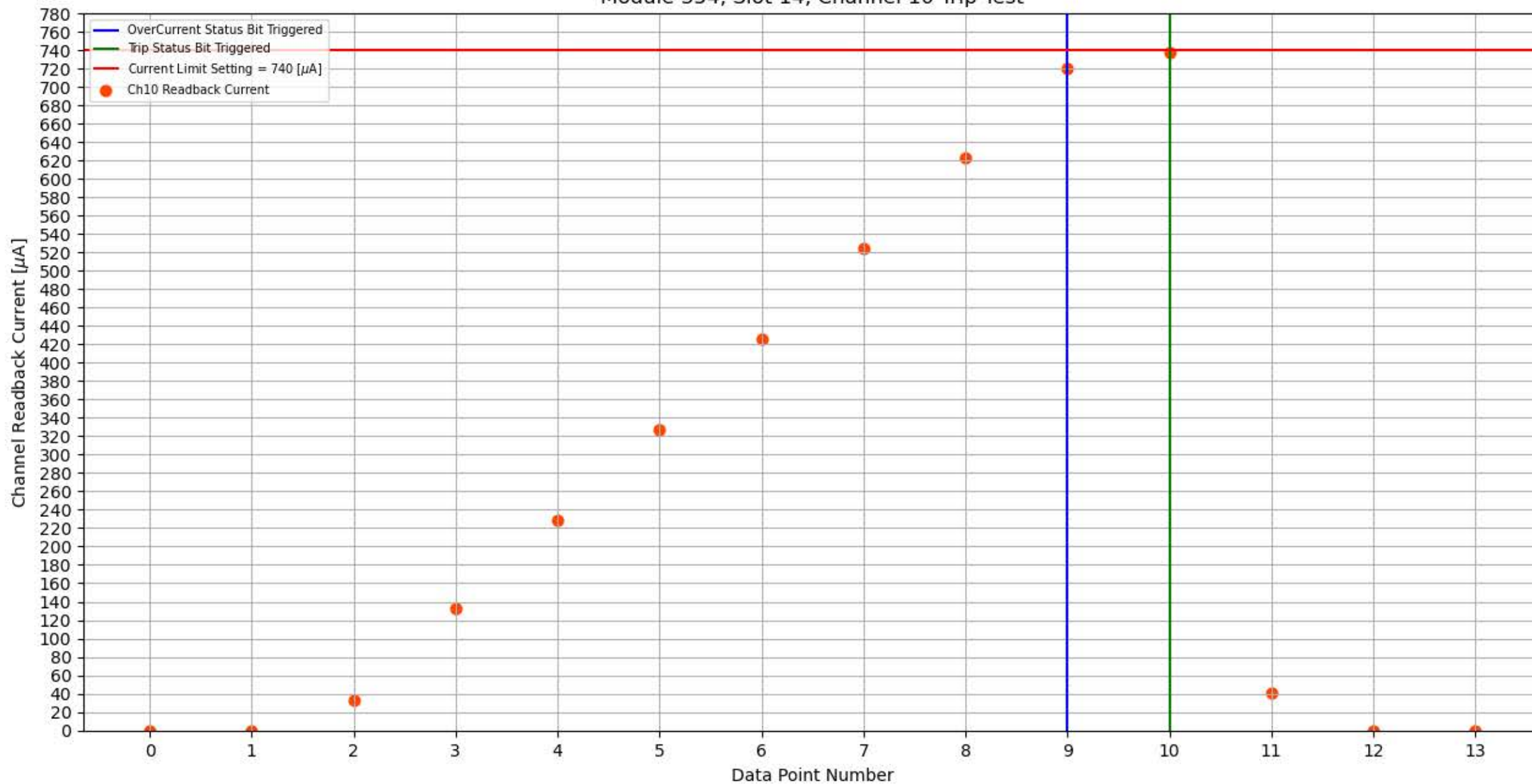
Module 354, Slot 14, Channel 10 Trip Test
