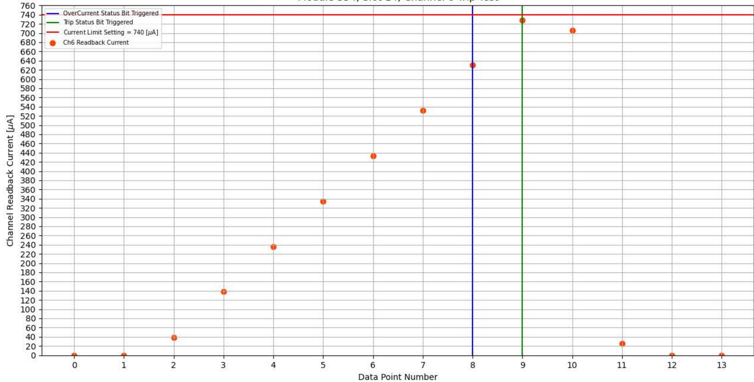
Module 354, Slot 14, Channel 6 Trip Test
