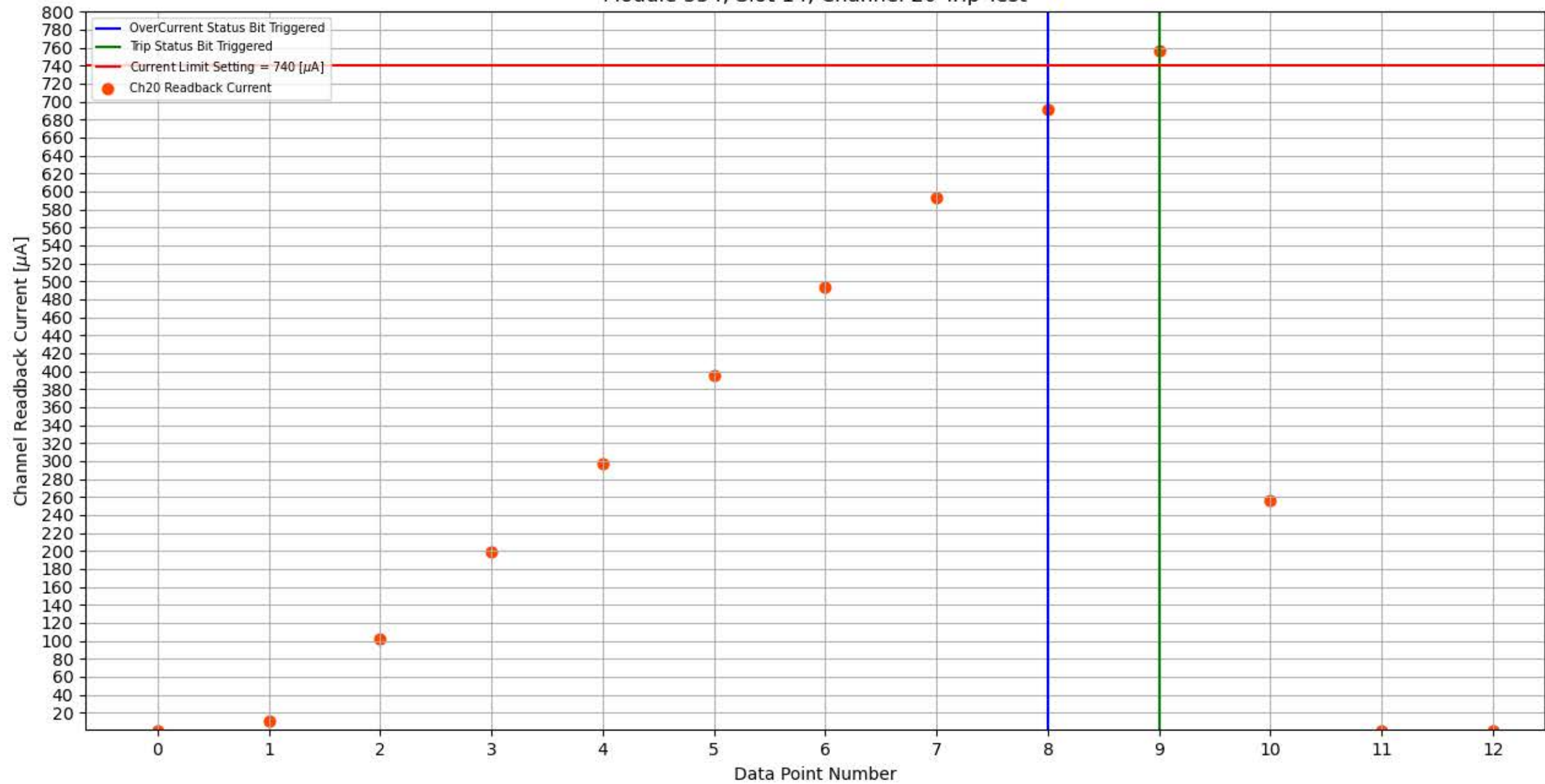
Module 354, Slot 14, Channel 20 Trip Test
