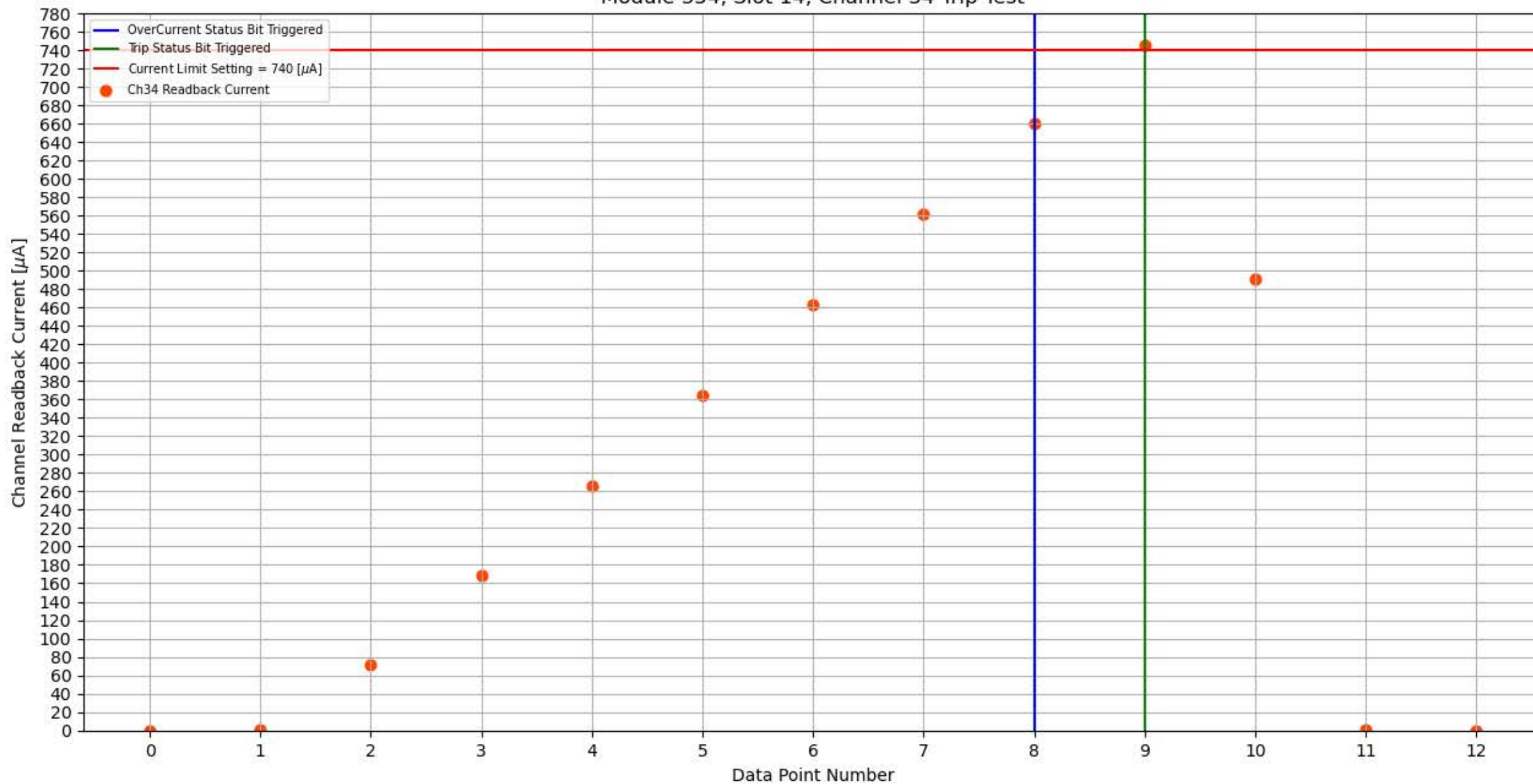
Module 354, Slot 14, Channel 34 Trip Test
