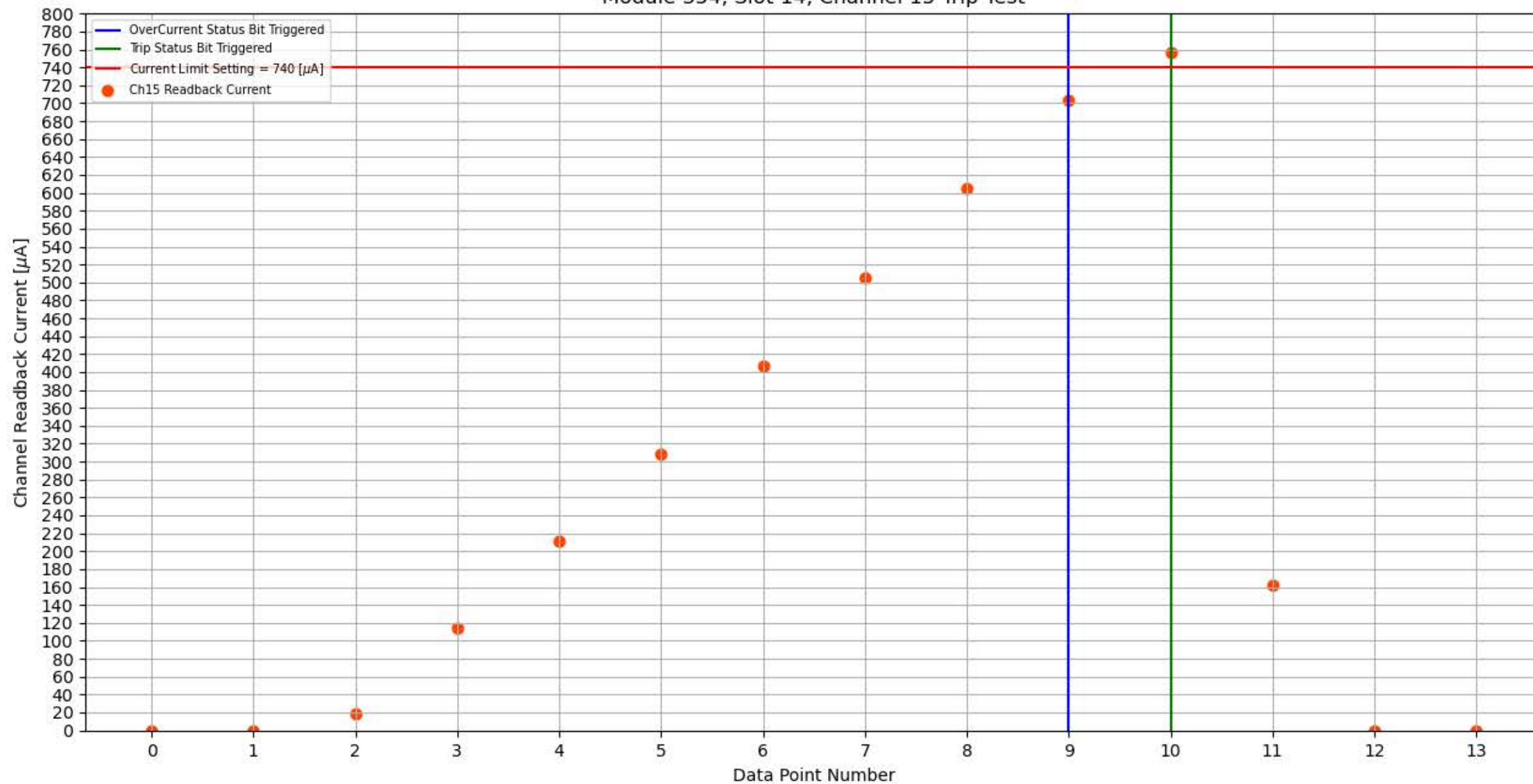
Module 354, Slot 14, Channel 15 Trip Test
