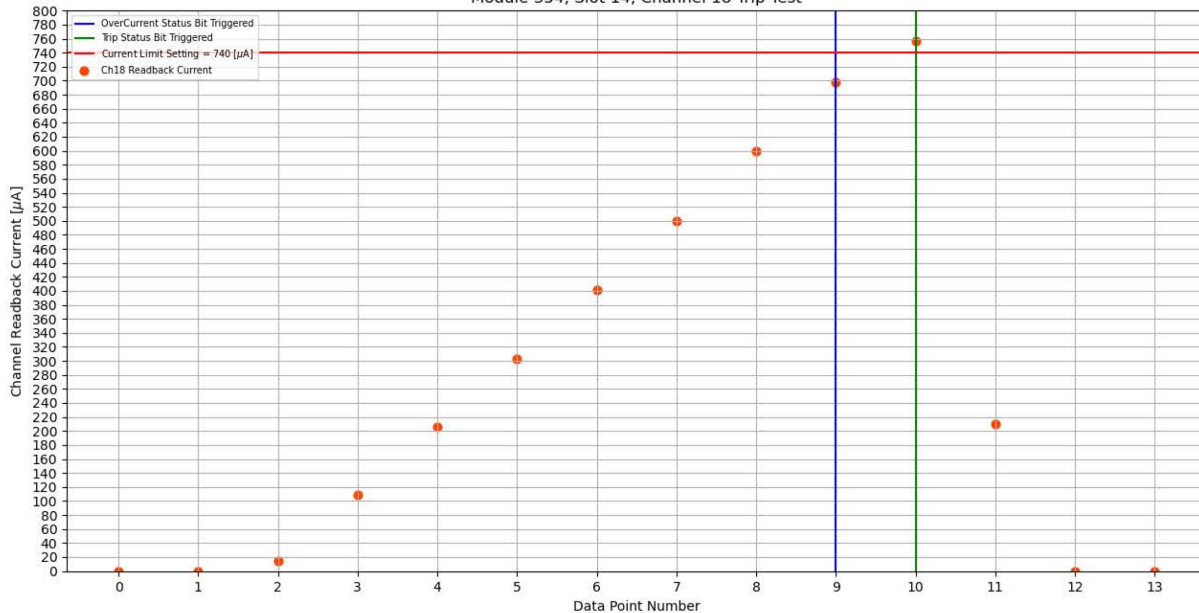
Module 354, Slot 14, Channel 18 Trip Test
