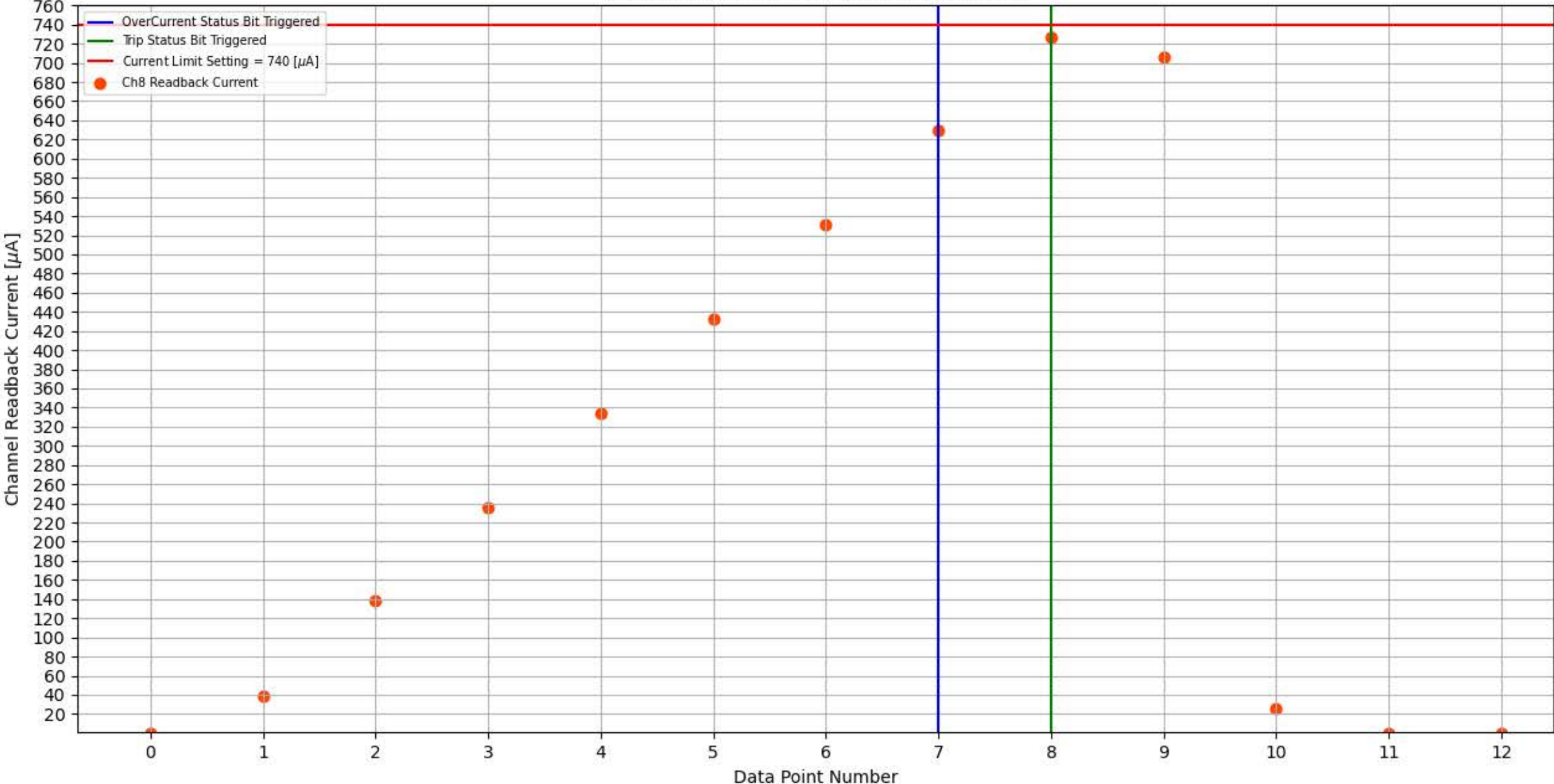
Module 354, Slot 14, Channel 8 Trip Test
