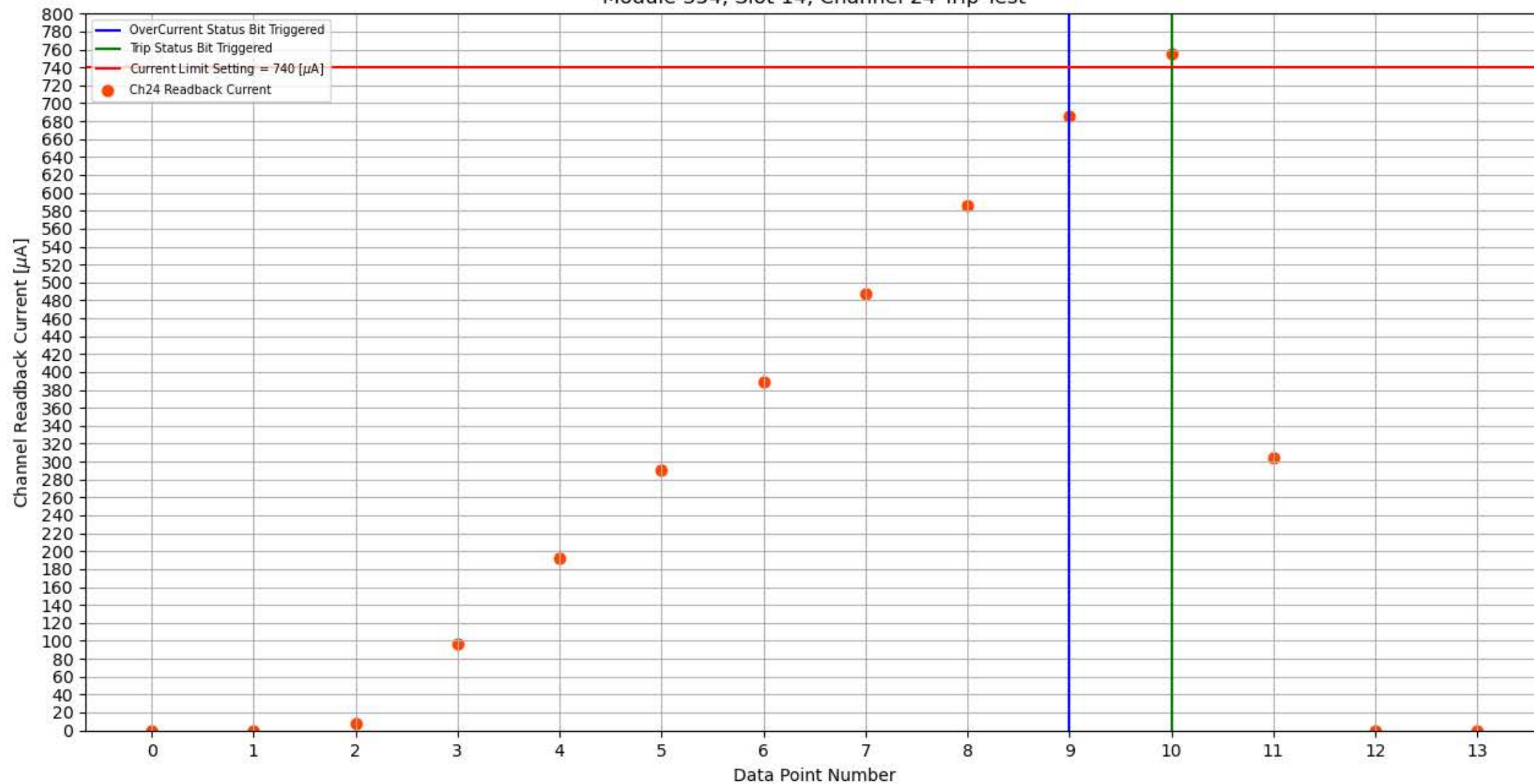
Module 354, Slot 14, Channel 24 Trip Test
