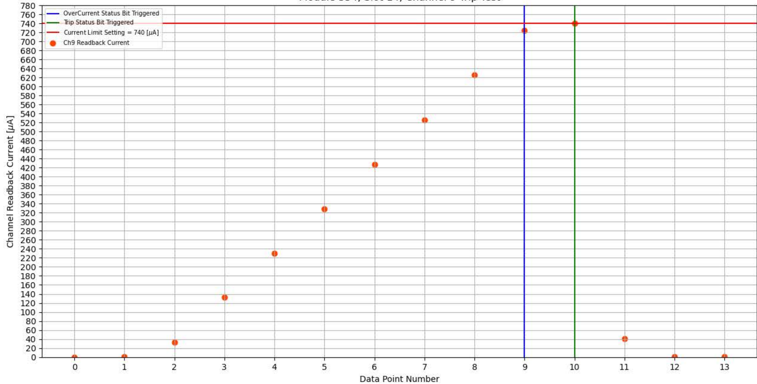
Module 354, Slot 14, Channel 9 Trip Test
