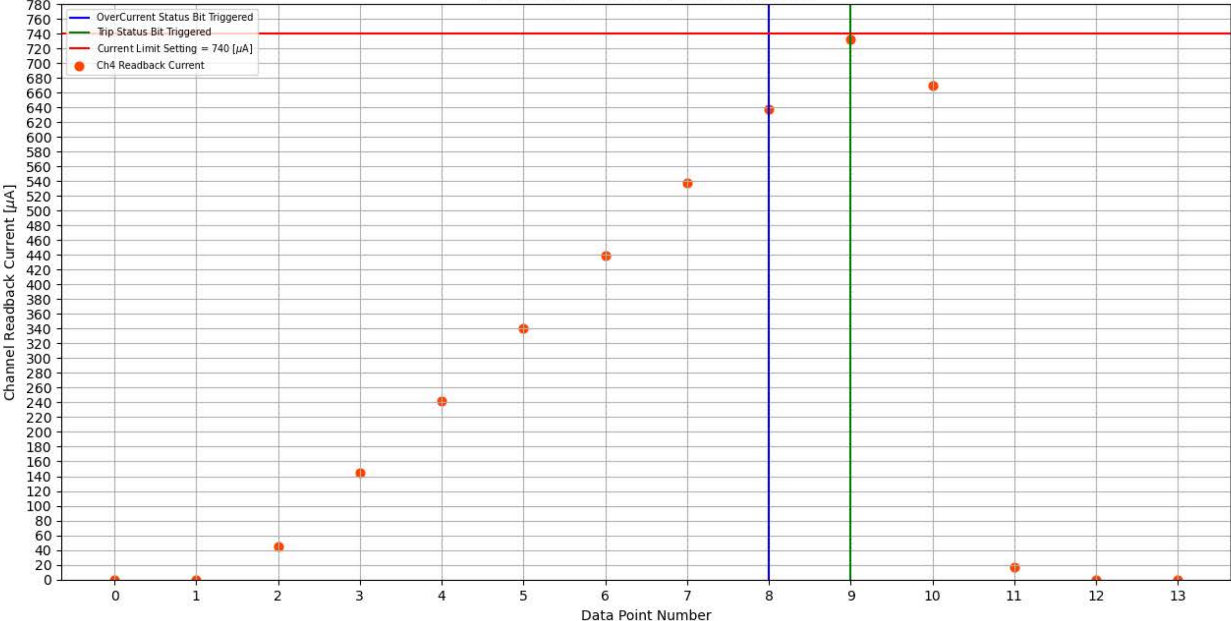
Module 354, Slot 14, Channel 4 Trip Test
