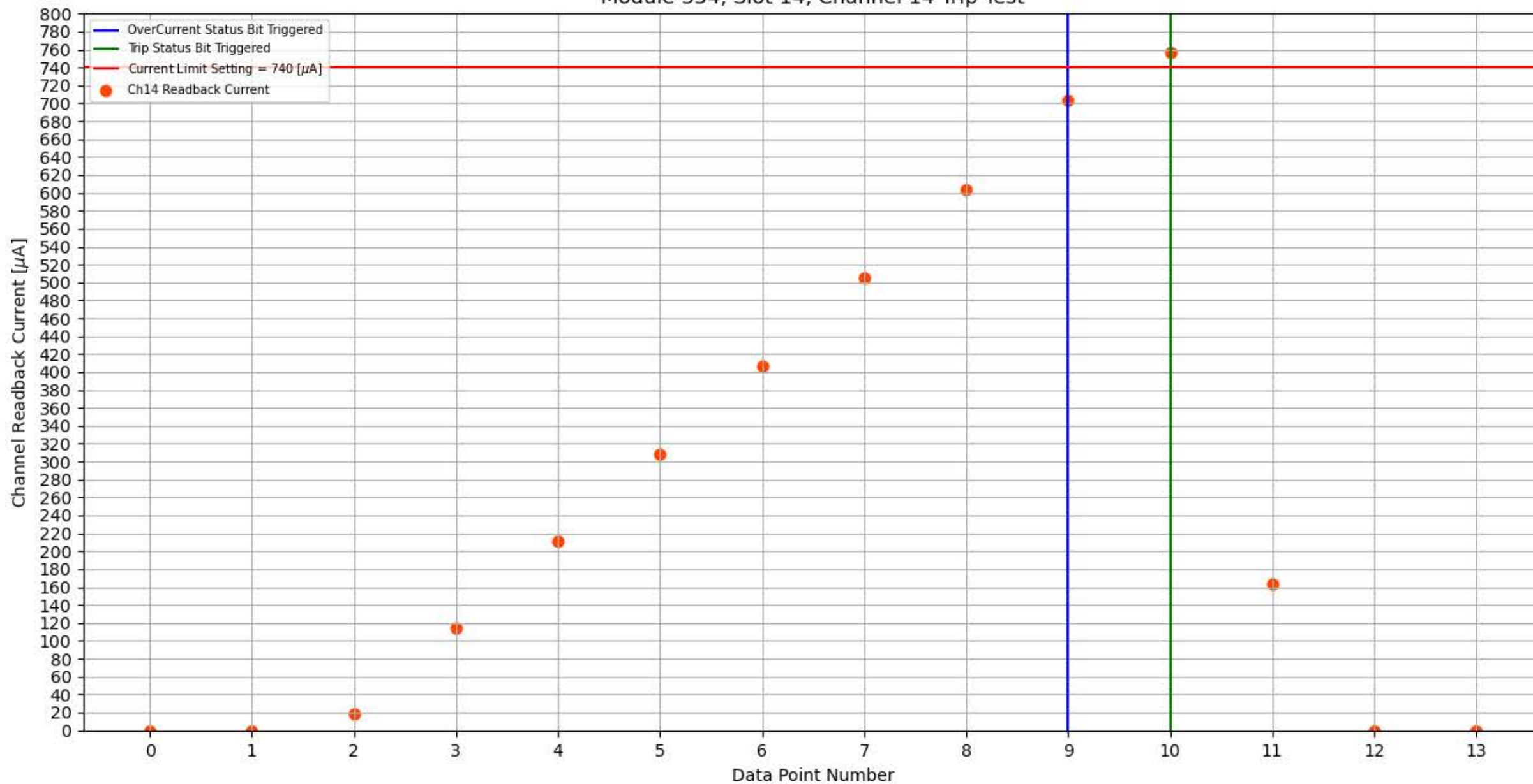
Module 354, Slot 14, Channel 14 Trip Test
