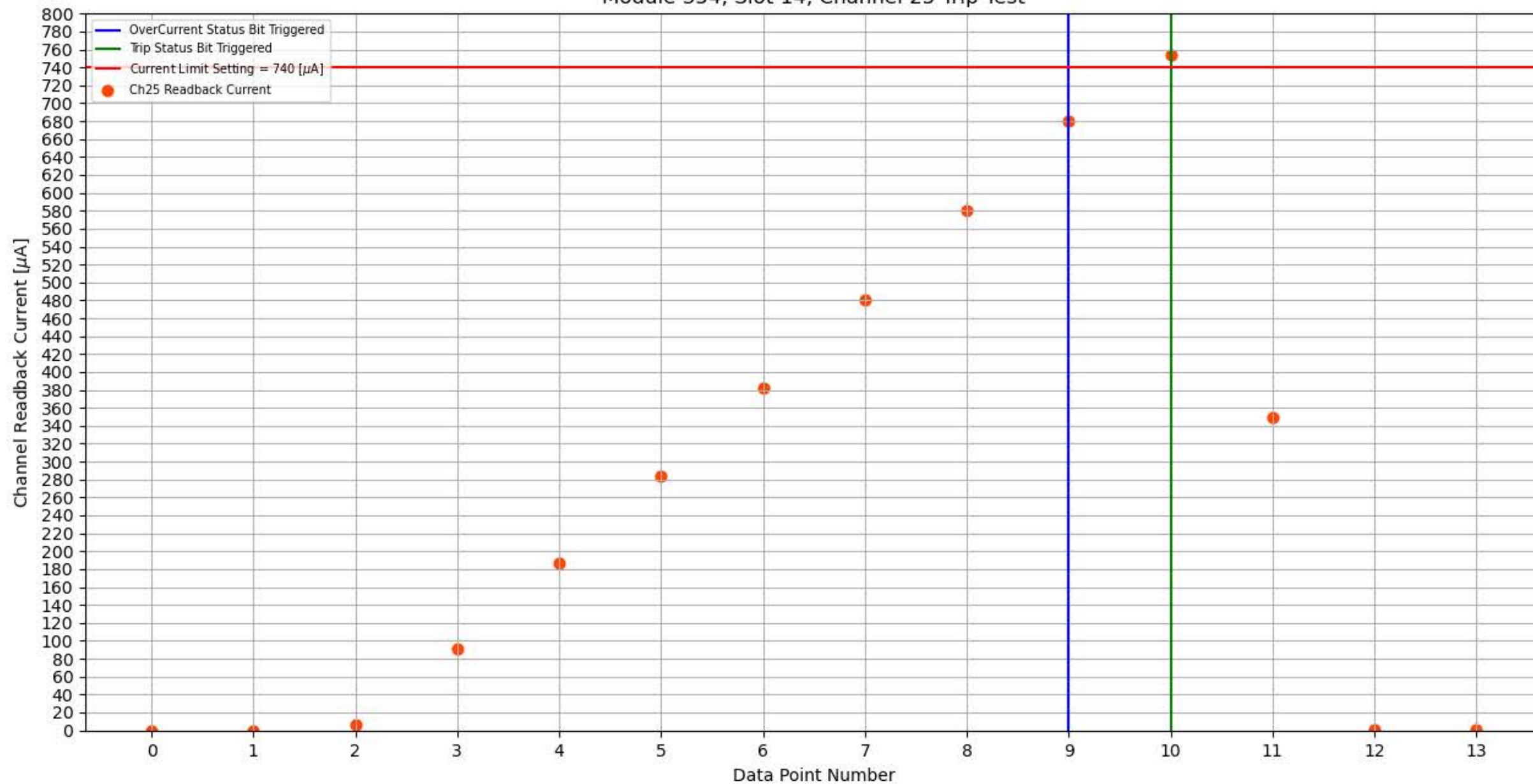
Module 354, Slot 14, Channel 25 Trip Test
