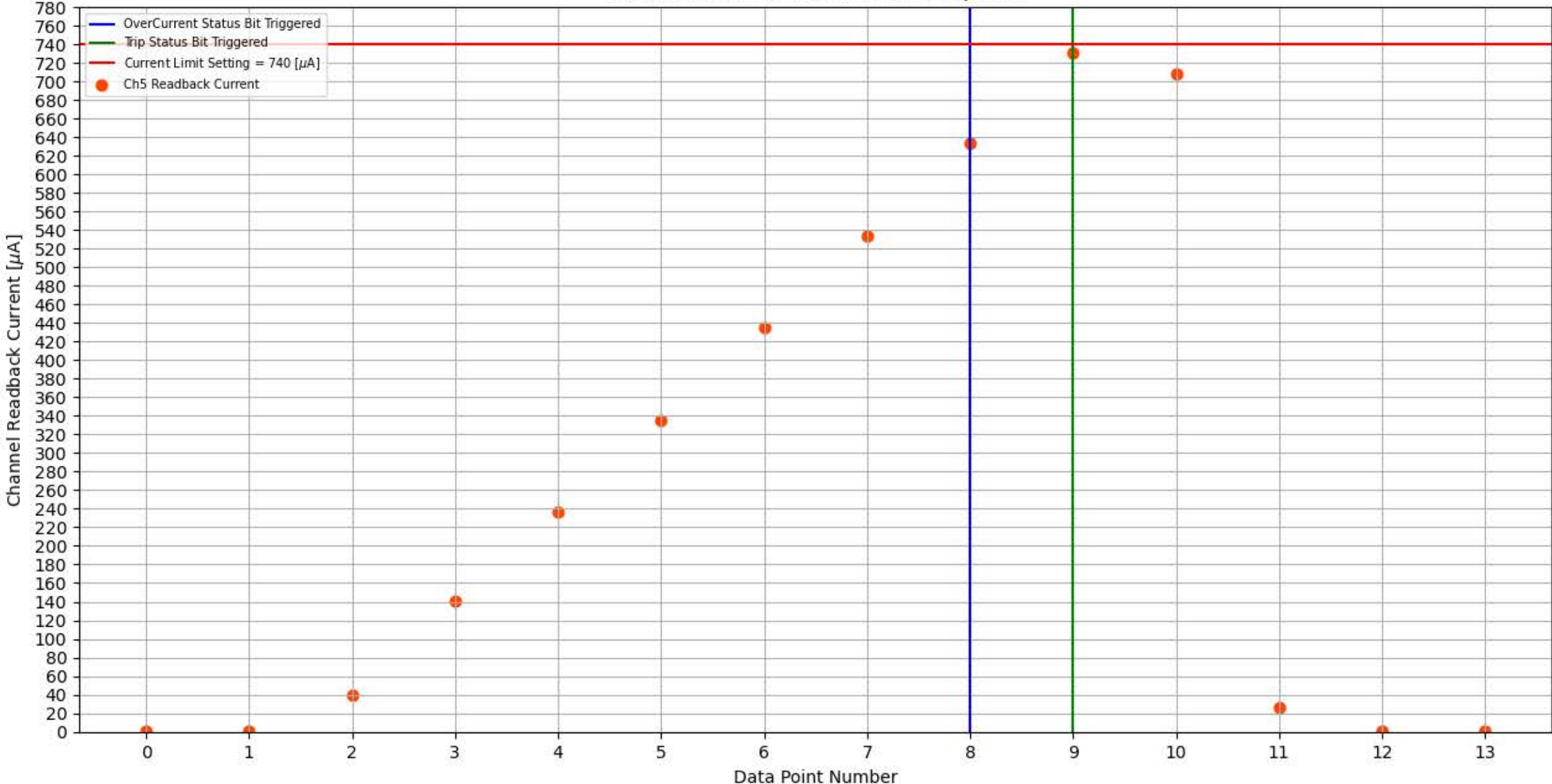
Module 354, Slot 14, Channel 5 Trip Test
