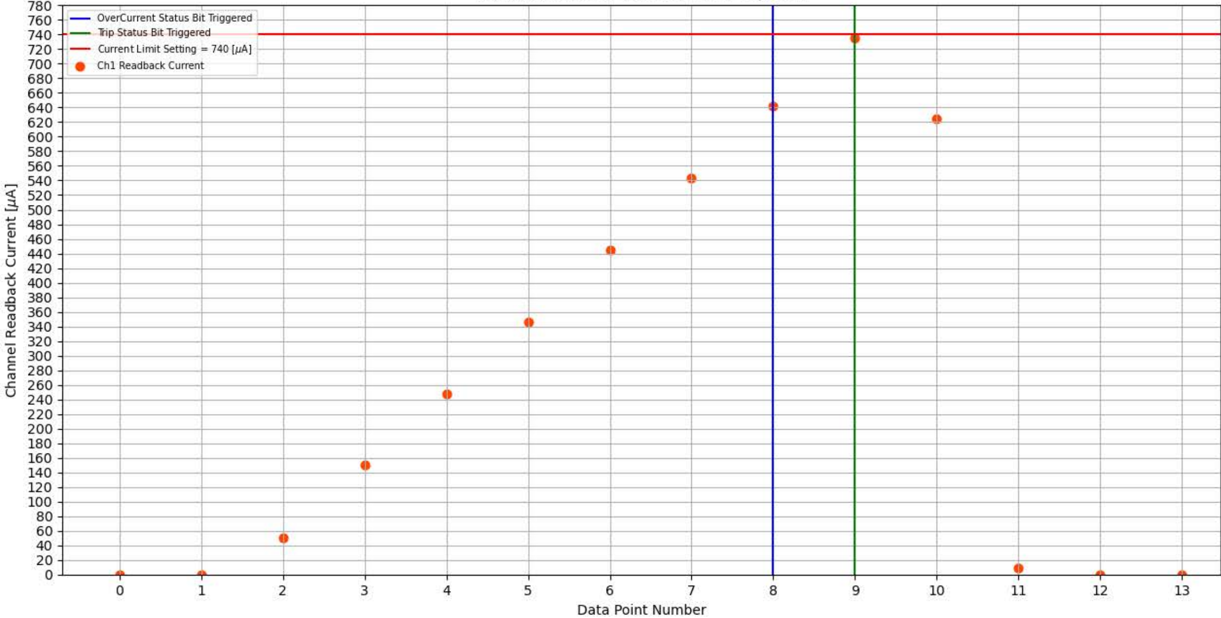
Module 354, Slot 14, Channel 1 Trip Test
