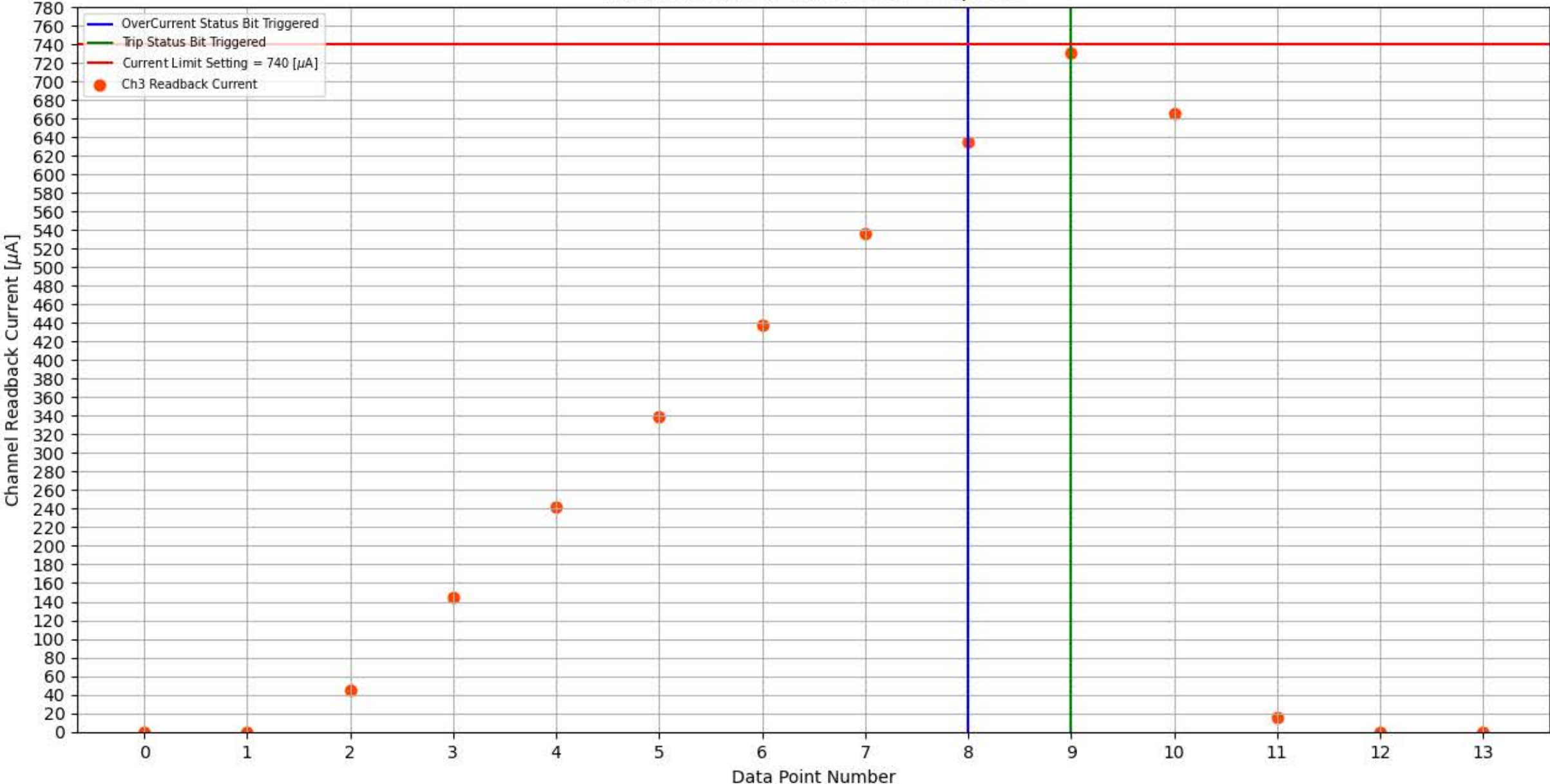
Module 354, Slot 14, Channel 3 Trip Test
