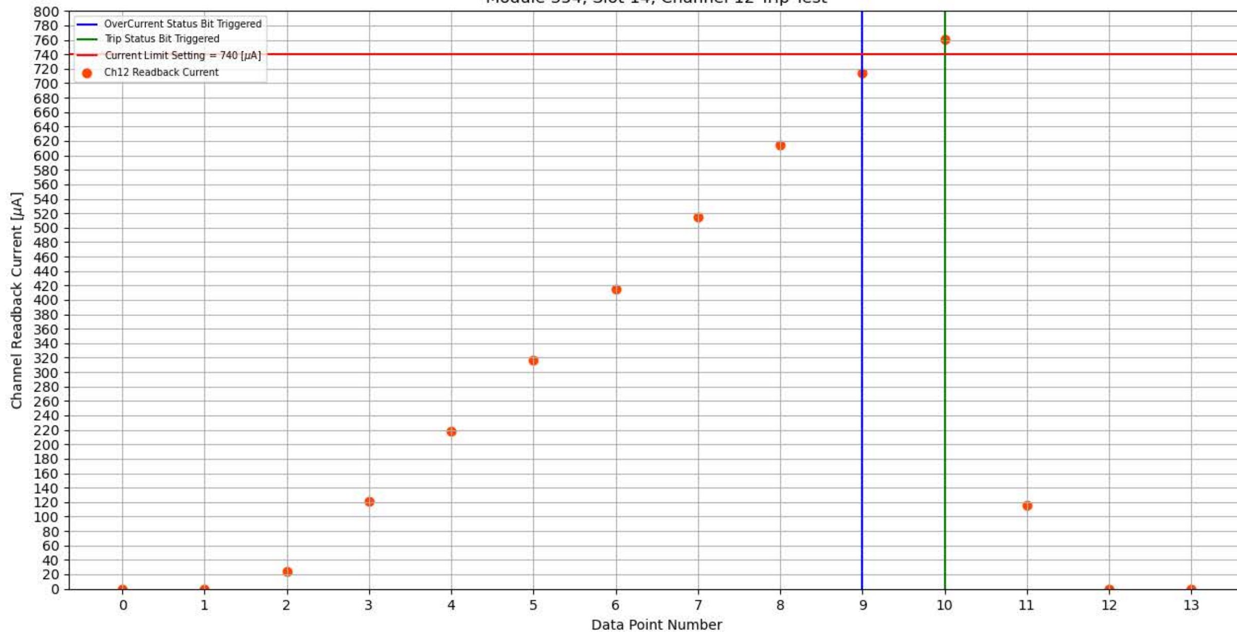
Module 354, Slot 14, Channel 12 Trip Test
