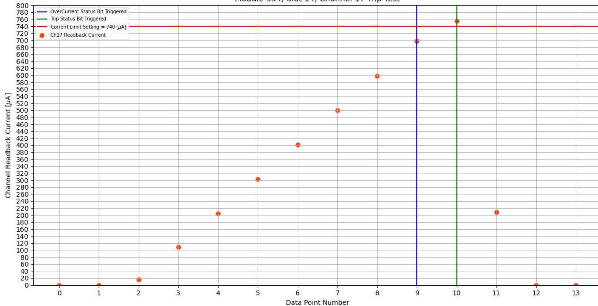
Module 354, Slot 14, Channel 17 Trip Test
