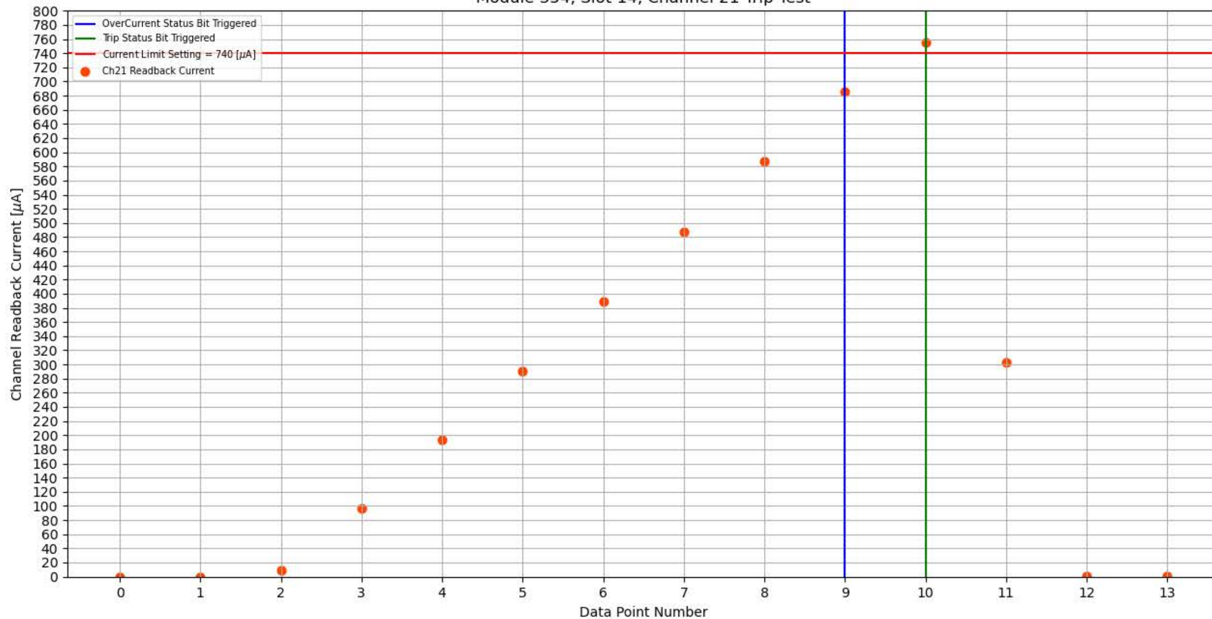
Module 354, Slot 14, Channel 21 Trip Test
