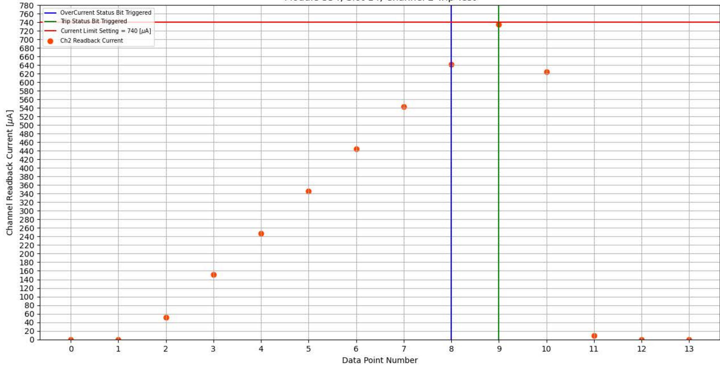
Module 354, Slot 14, Channel 2 Trip Test
