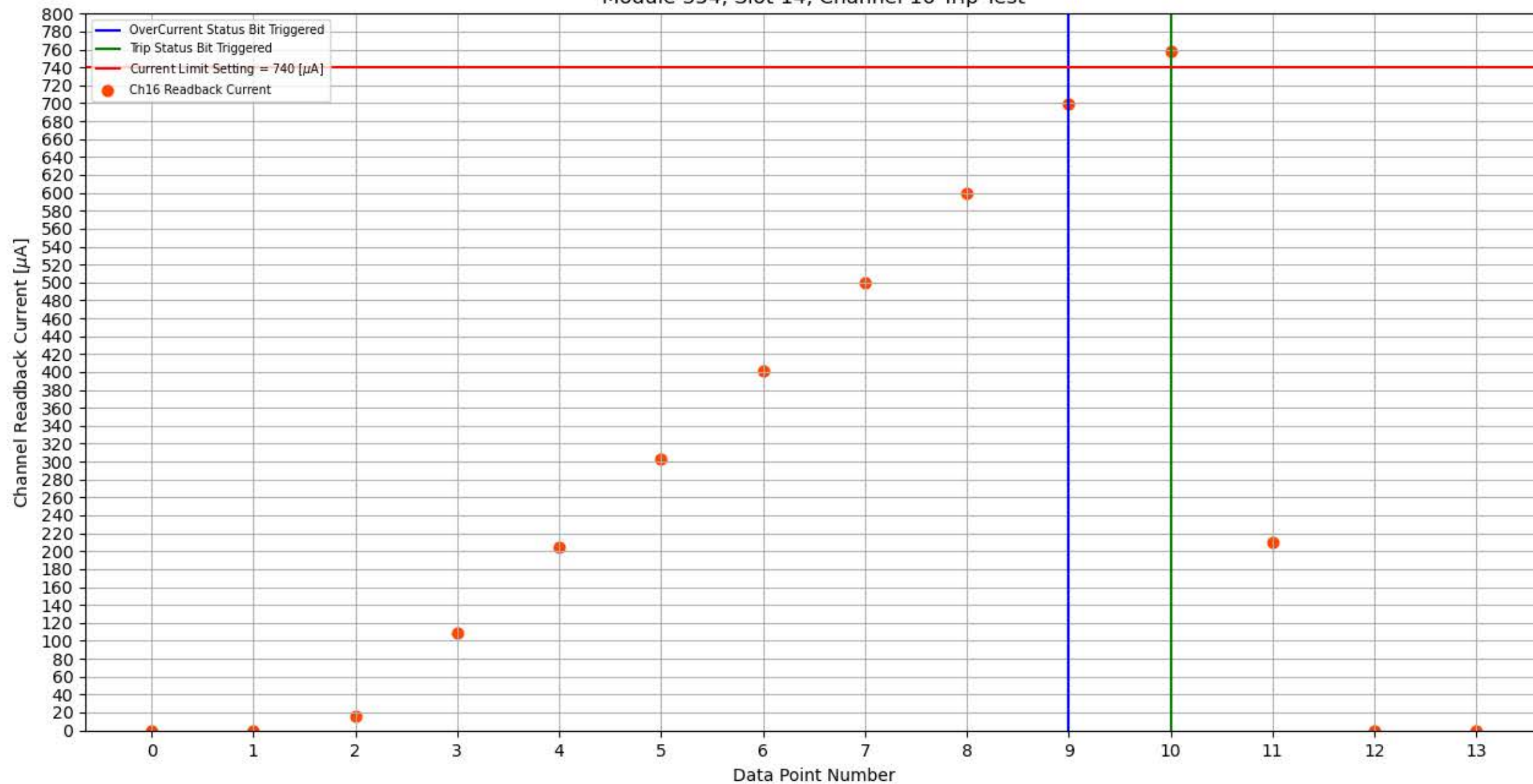
Module 354, Slot 14, Channel 16 Trip Test
