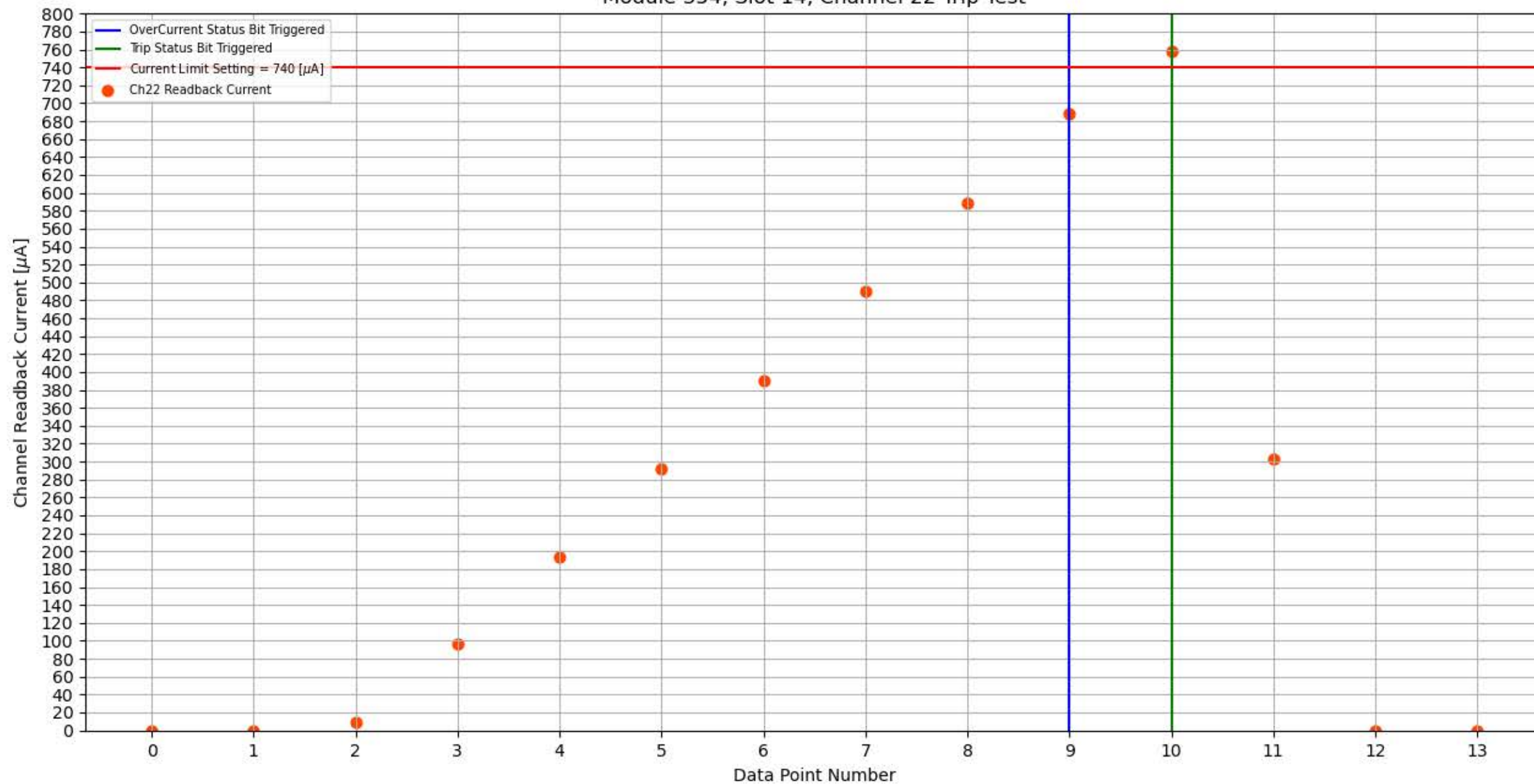
Module 354, Slot 14, Channel 22 Trip Test
